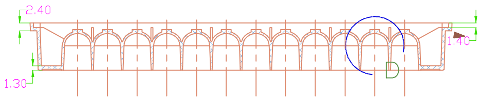
SECTION C-C
